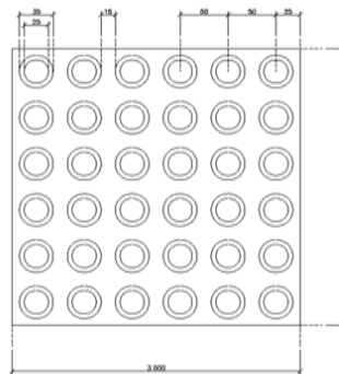
(a) Top view Figure F5 Warning Indicator
